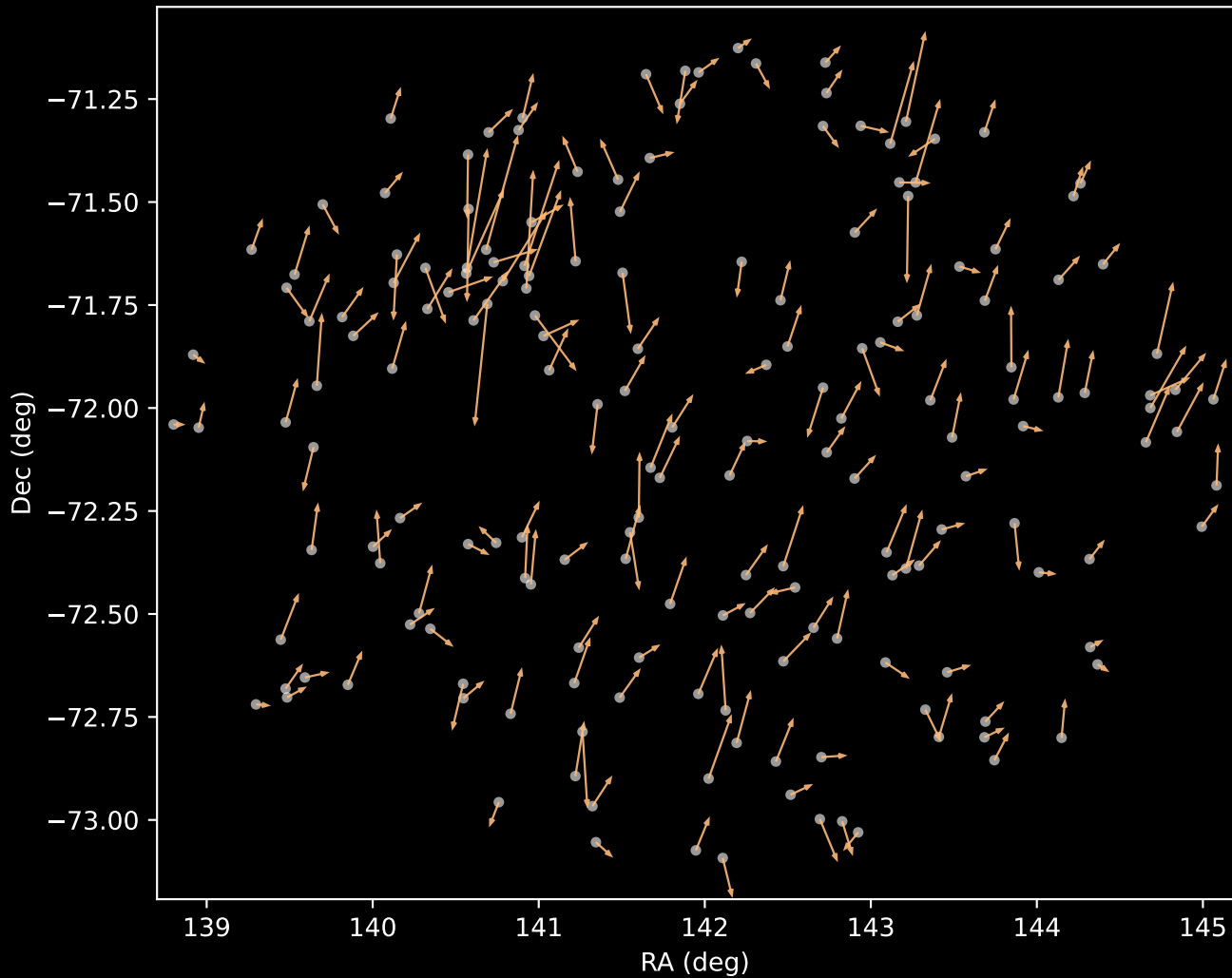
GALAH DR4 Cluster 3 Proper Motion Vectors (n=181)
