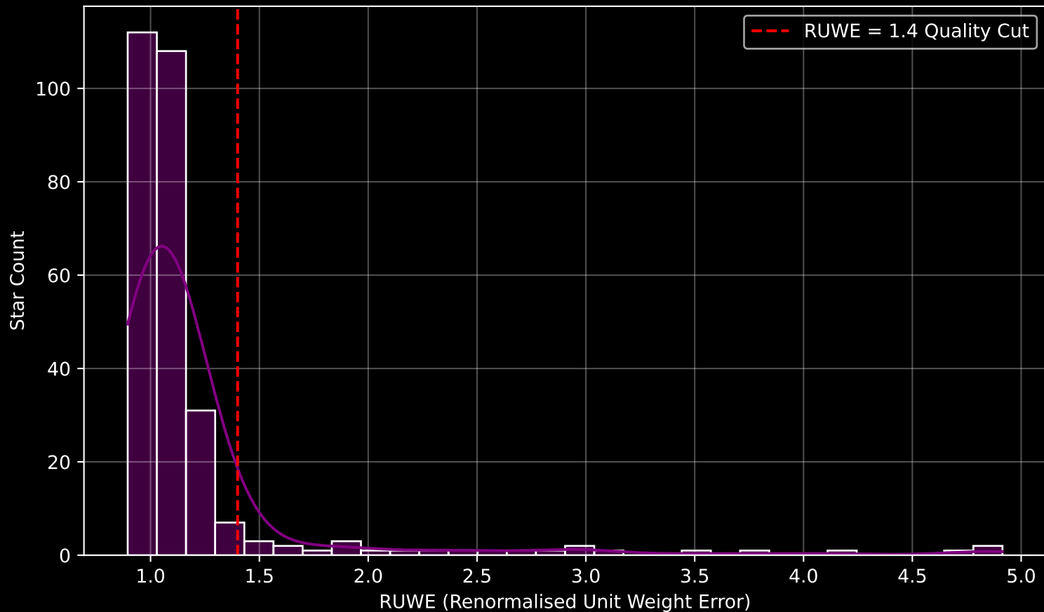
GALAH DR4 Field [131] RUWE Distribution (n= 283)
