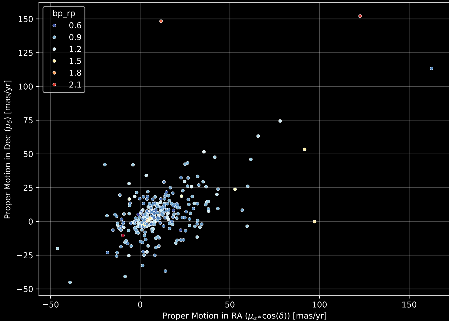
GALAH DR4 Field: [131] Proper Motion Diagram (n= 297)
