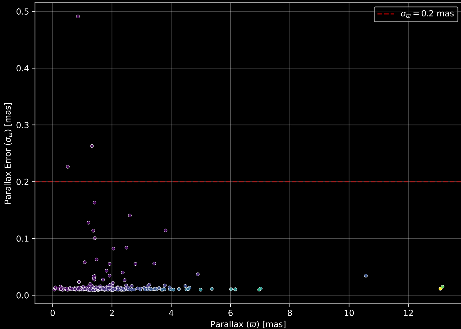
GALAH DR4 Field: [131] Parallax Quality (n= 297)
