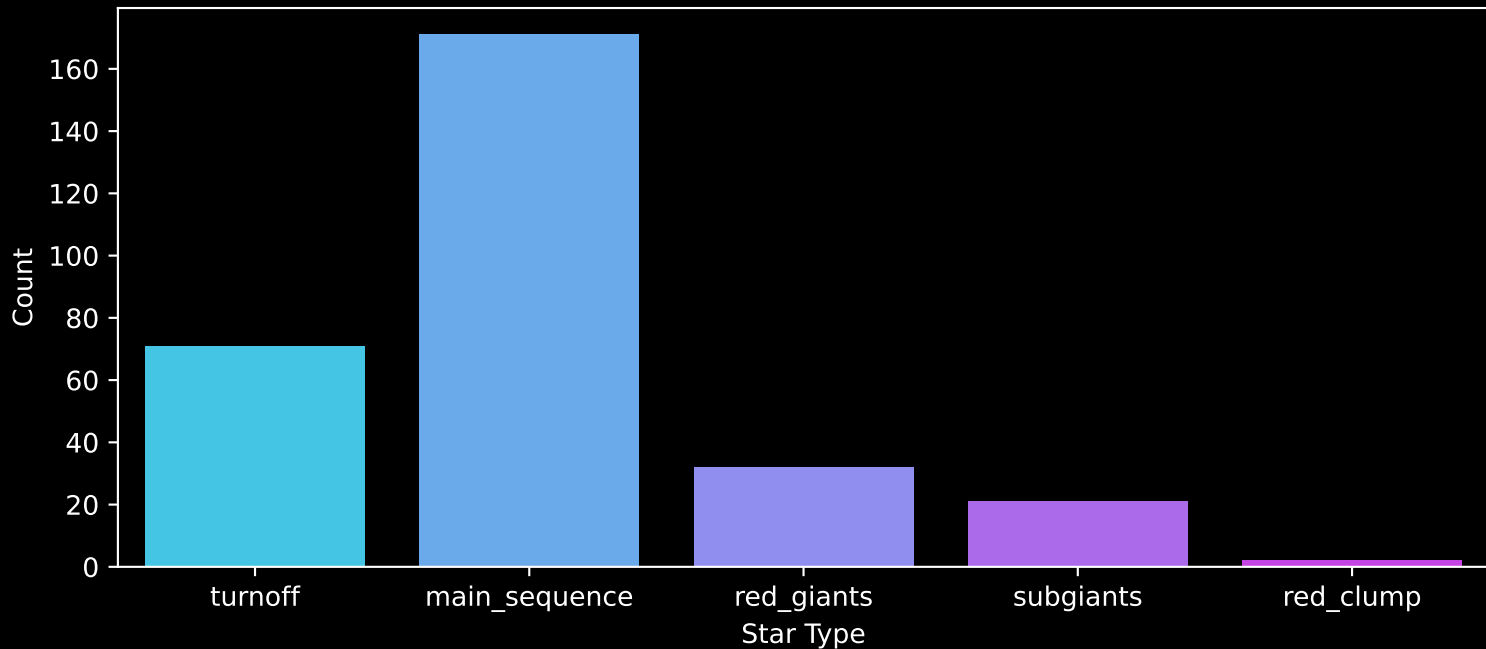
GALAH DR4 Field: [131] Count plot of Star Type
