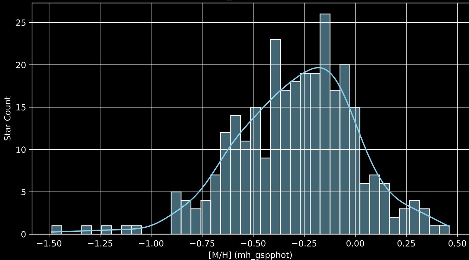
GALAH DR4 Field: [131] [M/H] (mh_gspphot) (n= 296)
